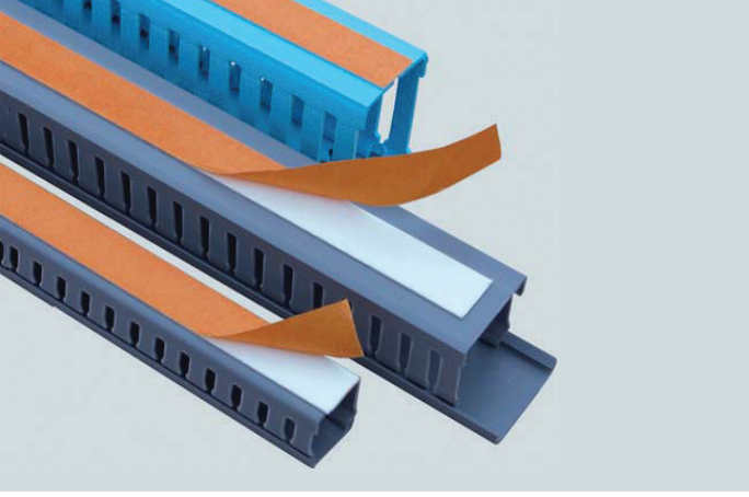
KOLAY YAPIŞMAYI SAĞLAYAN, ÇİFT TARAFLI BANT KULLANILABİLİR DOUBLE SIDED ADHESIVE TAPE ASSURING EASY FIXATION CAN BE USED
